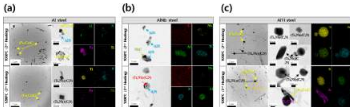
Fig. 6. (a) TEM image of Al steel, (b) AlNb steel, and (c) AlTi steel, each of which was 2nd solution-treated at both 1050°C and 1200°C.
