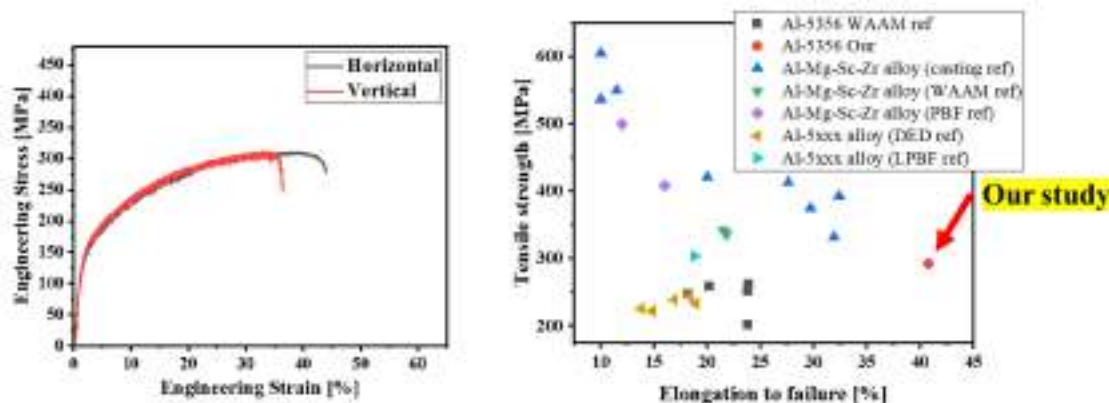
Fig. 2. (a) Tensile properties of WAAM 5356 with horizontal and vertical directions, (b) comparison of tensile properties with other reports.
