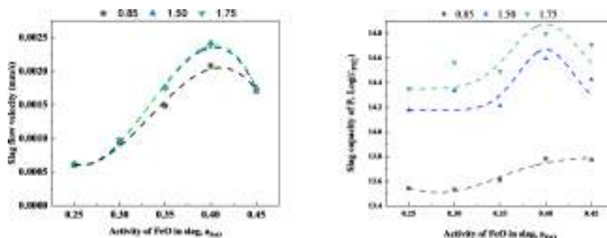
Fig. 2. Slag flow velocity (mm/s) , Phosphorus capacity( C_{PO_4^{3-}} )
