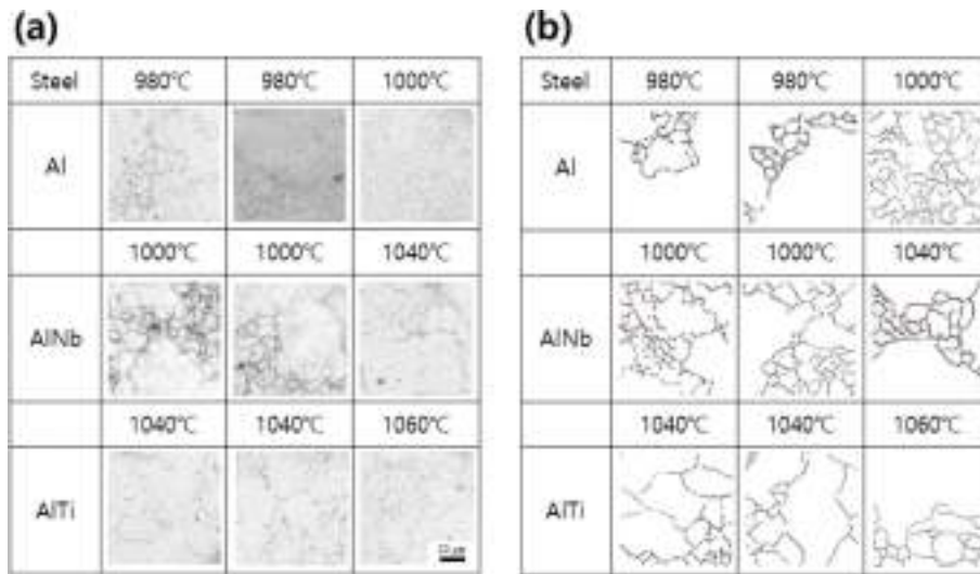
Fig. 10. Actual and generated austenite grain structure images of abnormal grain growth (AGG), for (a) actual and (b) generated austenite grain structure images.
