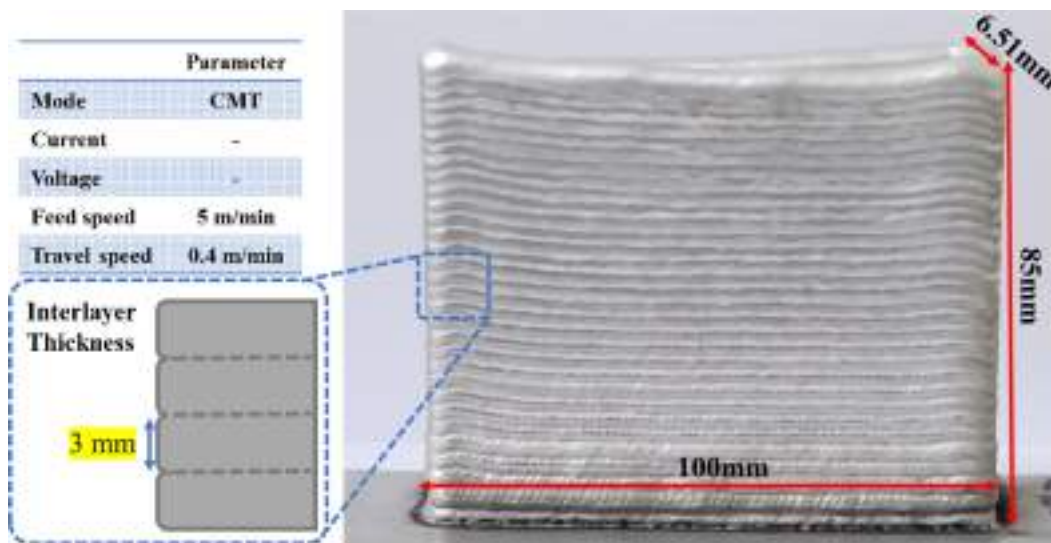
Fig. 1. Fabricated Al-5356 sample manufactured by wire arc additive manufacturing
