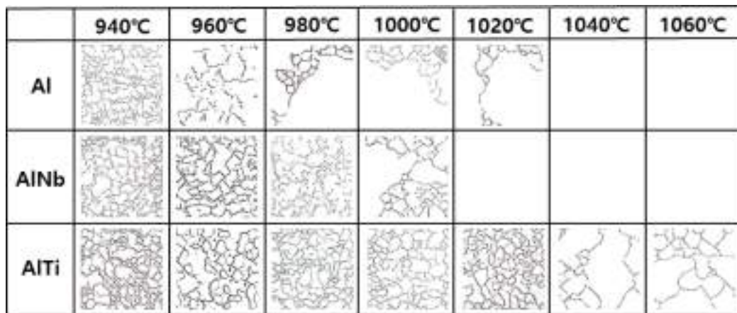
Fig. 8. Generated microstructure images using GAN at 3rd temperatures of 940-1080°C for 2nd temperature of 1150°C.
