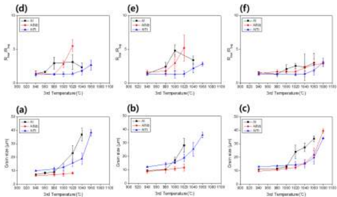
Fig. 4. Changes in (a-c) grain size and (d-f) R_{max}/R_{avg} with reheating temperature of Al and AlTi steels, which are 2nd reheating-treated at (a,d) 1050°C, (b,e) 1150°C, and (c,f) 1200°C.
