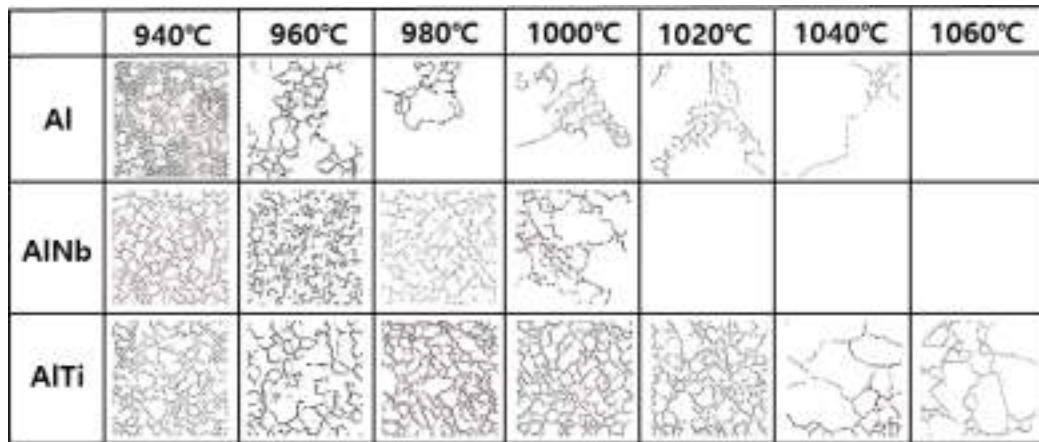
Fig. 7. Generated microstructure images using GAN at 3rd temperatures of 940-1080°C for 2nd temperature of 1050°C.
