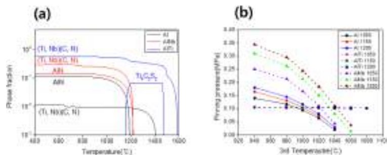
Fig. 3. Phase fraction of major precipitates and corresponding pinning pressure(MPa) for Al, AlNb, and AlTi steels.
