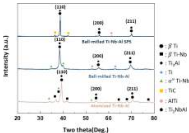
Fig. 2. Atomized Ti-Nb-Al, ball-milled Ti-Nb-Al, ball-milled Ti-Nb-Al SPS의 XRD 결과
