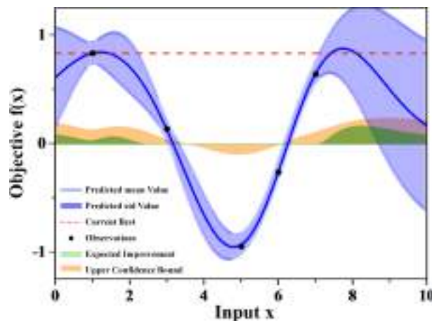
Fig. 2. Example of Upper confidence bound
