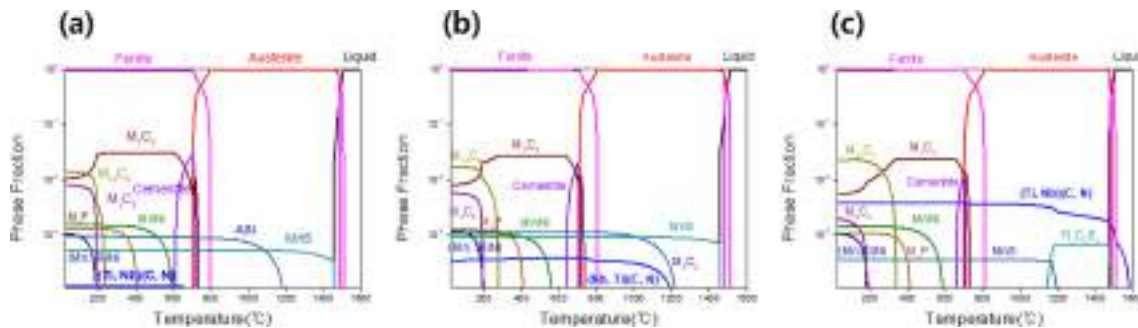
Fig. 1. Equilibrium phase fraction as a function of temperature for (a) Al steel and (b) AlNb steel and (c) AlTi steel.
