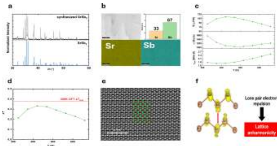
Fig. 1. (a) Powder XRD patterns of SrSb 2 measured at 298 K. (b) BSE-SEM images of polished surface of SrSb 2 with EDS mapping. Seebeck coefficient(S), electrical conductivity(σ), total thermal conductivity(κ tot ), and zT of samples are shown in (c) and (d). Atomic-resolution HAADF-STEM image of SrSb 2 showing its characteristic layered-chain structure. (e) Structural model of SrSb 2 is overlaid on the image for better visibility (Sr:Green, Sb:Brown). (f) Electron localization function map of SrSb 2 showing the existence of lone pair electrons whose repulsion is the origin of low lattice thermal conductivity.
