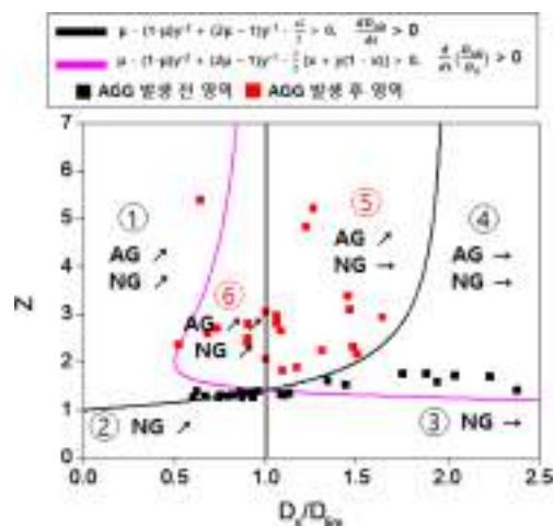
Fig. 5. Mapping diagram of abnormal grain growth (AGG) conditions.
